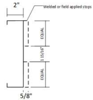
3 Head Detail Example (NTS)
