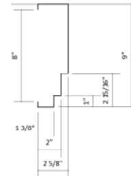
180 DEGREE JAMB DETAIL
