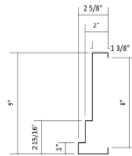
90 DEGREE JAMB DETAIL
