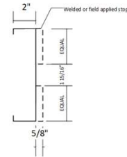
3 Head Detail Example (NTS)
