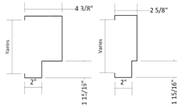
2 Jamb / Head Detail Example (NTS)
