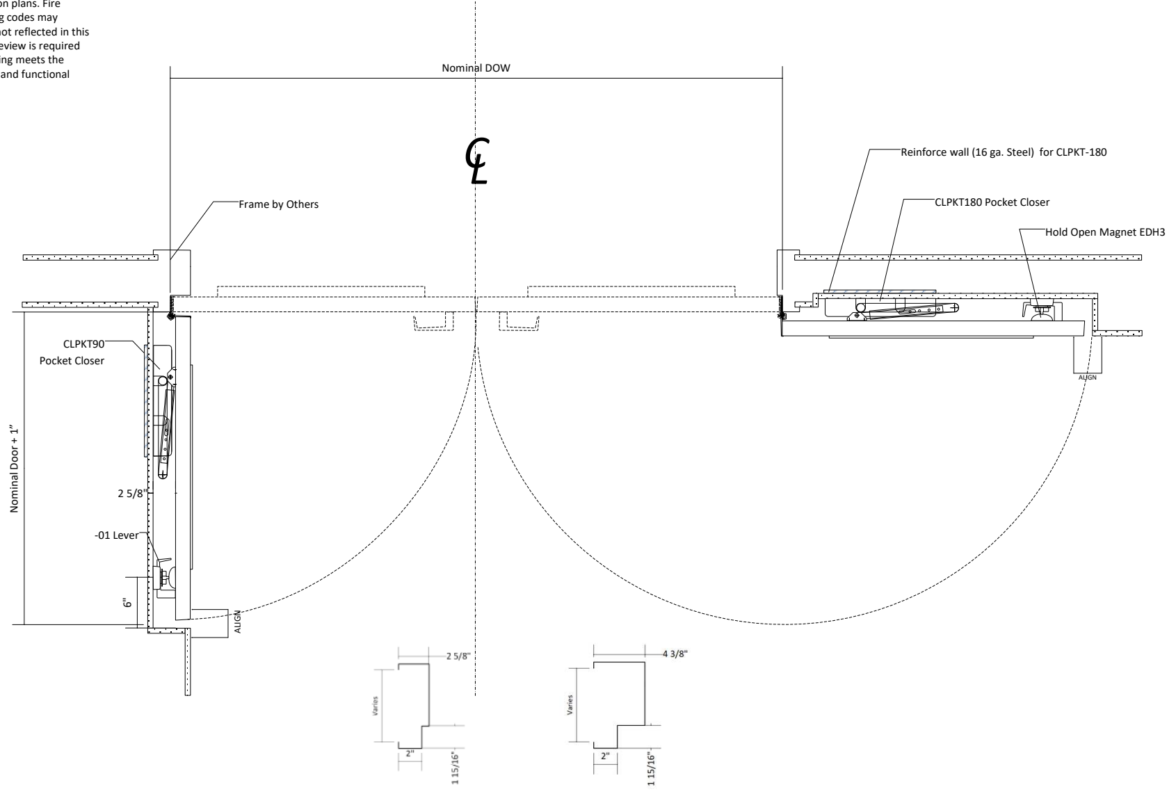
2 180° Door Jamb/ Head Detail Example (NTS)
