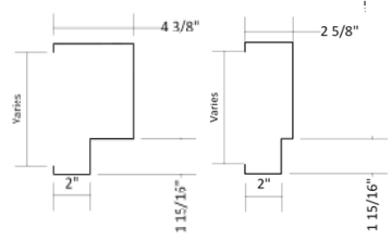
2 Jamb / Head Detail Example (NTS)
