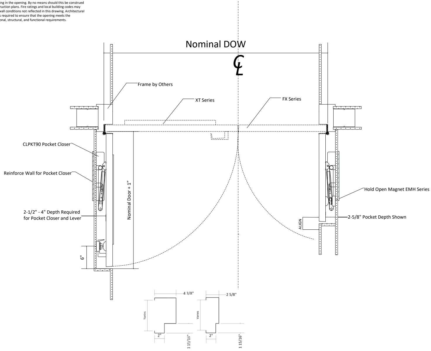
2 Jamb / Head Detail Example (NTS)
