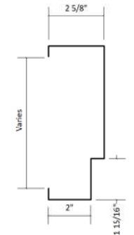
Head/Latch-side Jamb
