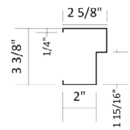
2 Head/Jamb Detail NTS
